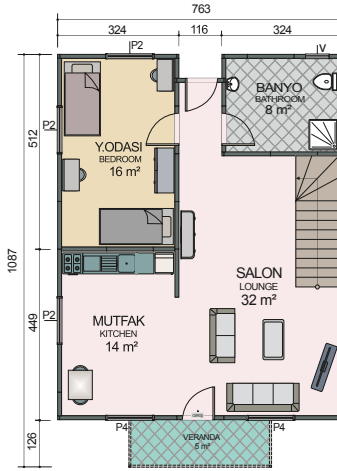
Zemin Kat Planı Ground Floor Plan 74m 2 + 5m 2 = 79m 2
