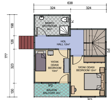
1. Kat Planı First Floor Plan 41\text{m}^2 + 4\text{m}^2 = 45\text{m}^2
