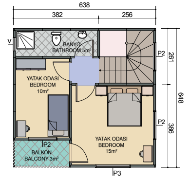
1. Kat Planı First Floor Plan 38\text{m}^2 + 3\text{m}^2 = 41\text{m}^2
