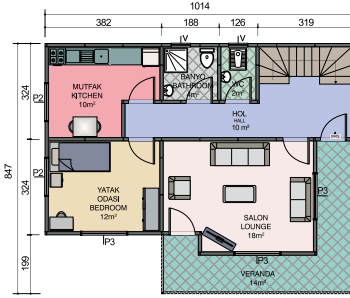
Zemin Kat Planı Ground Floor Plan 64m 2 + 14m 2 = 78m 2
