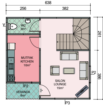
Zemin Kat Planı Ground Floor Plan 38\text{m}^2 + 3\text{m}^2 = 41\text{m}^2
