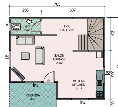
Zemin Kat Planı Ground Floor Plan 45\text{m}^2 + 7\text{m}^2 = 52\text{m}^2
