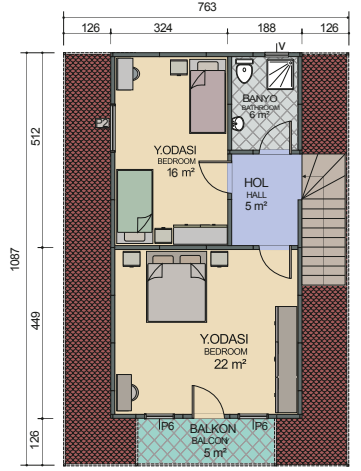
1. Kat Planı First Floor Plan 50m 2 + 5m 2 = 55m 2
