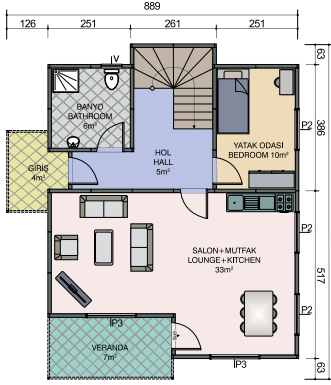
Zemin Kat Planı Ground Floor Plan 64m^2 + 11m^2 = 75m^2
