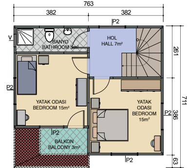
1. Kat Planı First Floor Plan 45\text{m}^2 + 3\text{m}^2 = 48\text{m}^2
